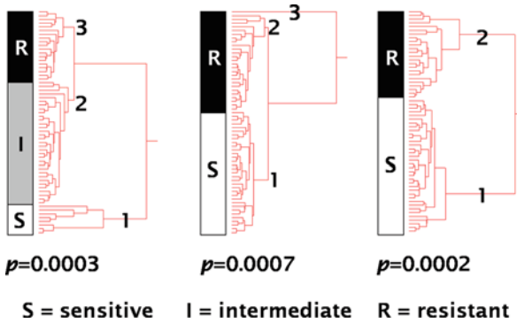
Fig. 22.2 Dendrograms of hierarchical cluster analysis (complete linkage method) obtained from mRNA expression of genes correlating with \log_{10} IC_{50} values for doxorubicin (a), vincristine (b), or methotrexate (c). The dendrograms show the clustering of 60 cell lines of the NCI's screening panel according to the mRNA expression profile of each 50 genes for each of the three drugs identified by COMPARE analysis. p values from \chi^2 tests are given
