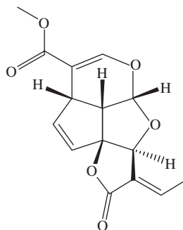
Plumericin
