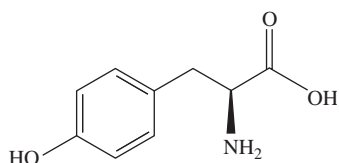
(S)-(-)-Tyrosine
