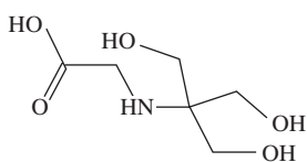
Tricine
