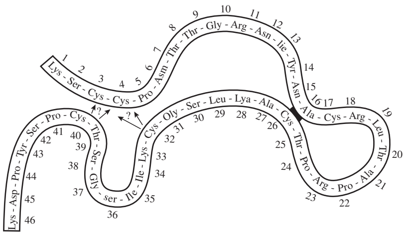
Viscotoxin A3
